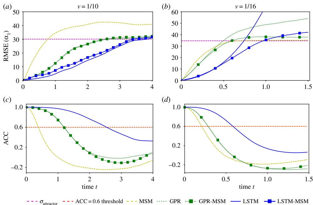
Figure 9. (a,b) RMSE evolution of the most energetic mode of the K-S equation with 1/\nu = 10 and 1/\nu = 16 . (c, d) ACC evolution of the most energetic mode of the K-S equation with 1/\nu = 10 and 1/\nu = 16 (in all plots, average value over 1000 initial conditions is reported). (Online version in colour.)
